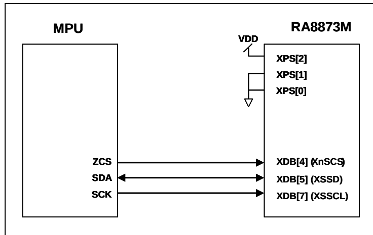
圖 7-7 : The MPU Interface Diagram of 3-Wire SPI
